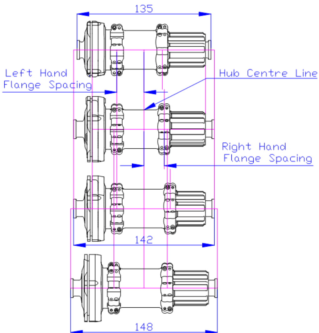
Figure 2: Illustrating Road, Mountain Bike Standard, Jump Bike and Mountain Bike Boost versions of KOM Xeno Hubs and different length cassette holder options. Hubs aligned with all hub CENTRE lines.
